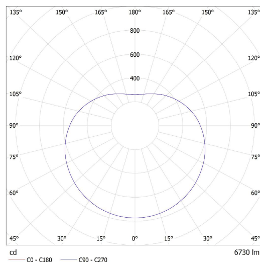
Lucis ZK.P1.600.X POLARIS ZK LED / LDC (Polar)
